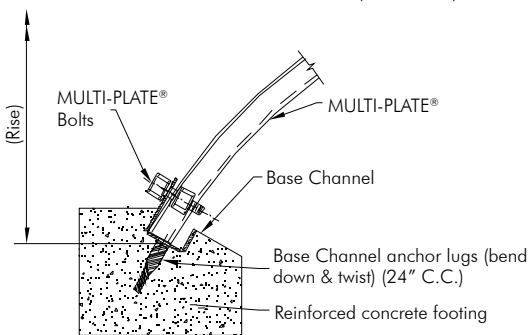
Steel Base Channel Example
