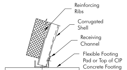
Aluminum Receiving Channel Example
